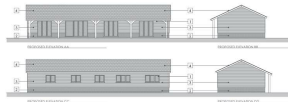
PROPOSED ELEVATIONS
